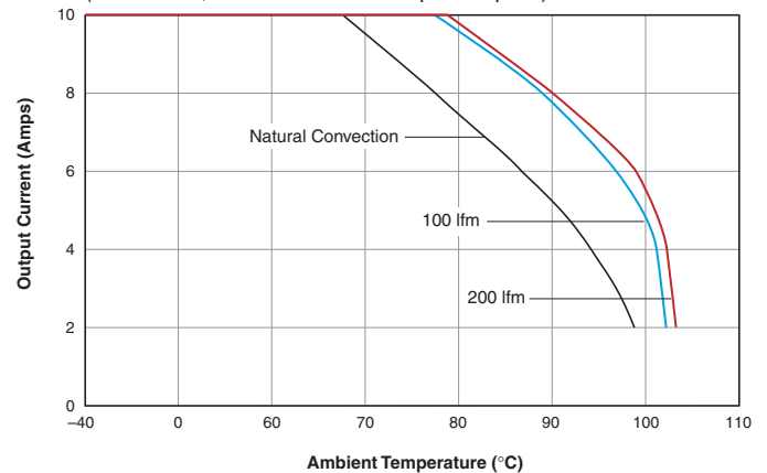
LSM-1.5/10-D5 Output Current vs. Ambient Temperature (SMT mount, air flow direction from pin 2 to pin 1)
