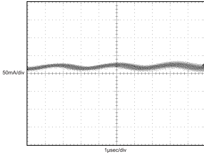
Input Reflected Ripple Current (Input Filter = 220μF/12μH/33μF, IOUT = 3.3V/10A)
