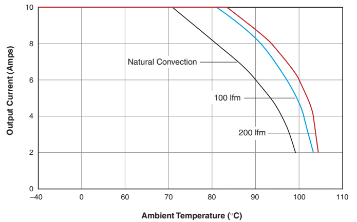
LSM-1/10-D5 Output Current vs. Ambient Temperature (SMT mount, air flow direction from pin 2 to pin 1)
