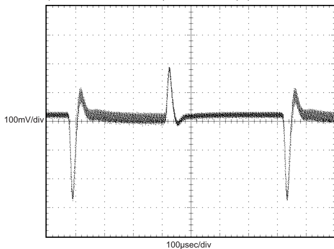
Dynamic Load Response
