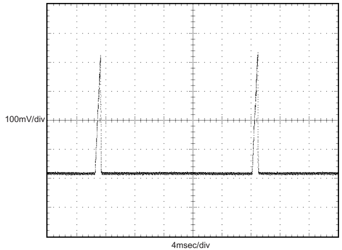
Output Hiccup (LSM-3.3/10-D5 Shorted VOUT)
