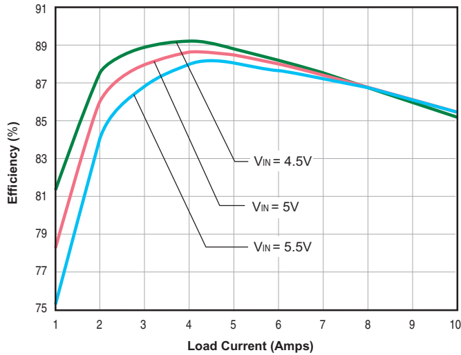
LSM-1.2/10-D5 Efficiency vs. Line Voltage and Load Current
