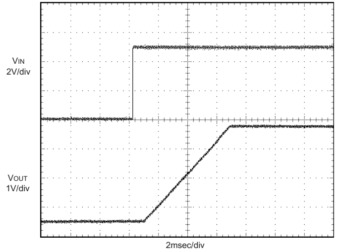
Start-Up from VIN (IOUT = 3.3V/10A, CIN/COUT = 22μF)
