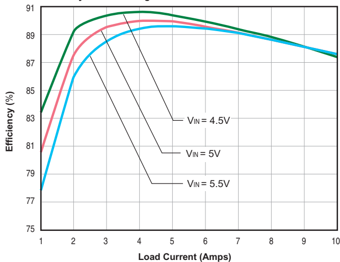
LSM-1.5/10-D5 Efficiency vs. Line Voltage and Load Current
