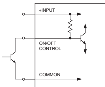
ON/OFF pin open: Logic High = DC/DC converter On ON/OFF pin <0.4V: Logic Low = DC/DC converter Off
