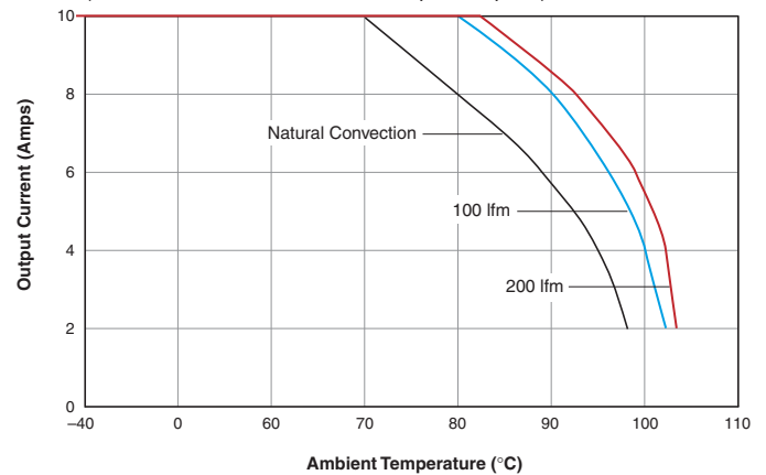
LSM-1.2/10-D5 Output Current vs. Ambient Temperature (SMT mount, air flow direction from pin 2 to pin 1)
