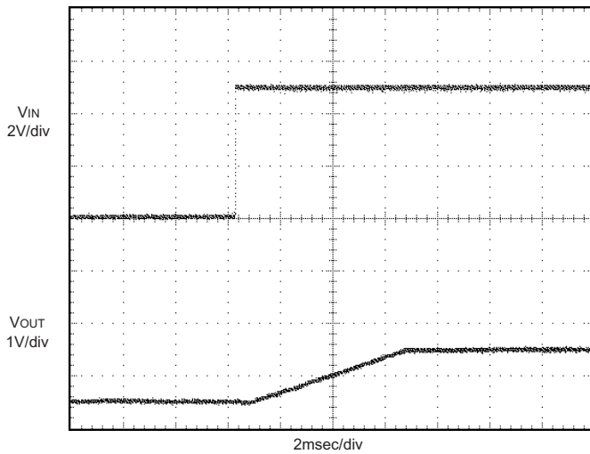
Start-Up from VIN (IOUT = 1V/10A, CIN/COUT = 22μF)
